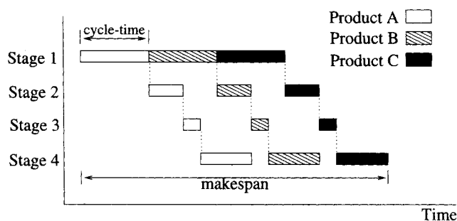
Figure 1. Gantt plot of single-product campaign (SPC) with overlapping operation.
